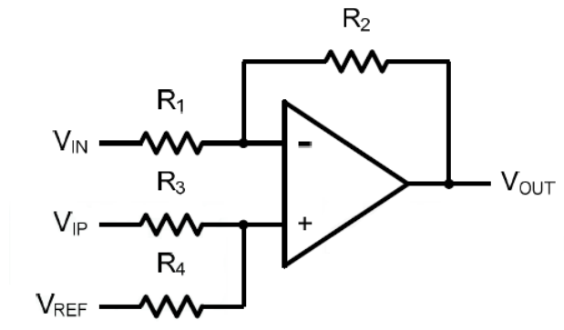
Figure 3. Differential Amplifier
