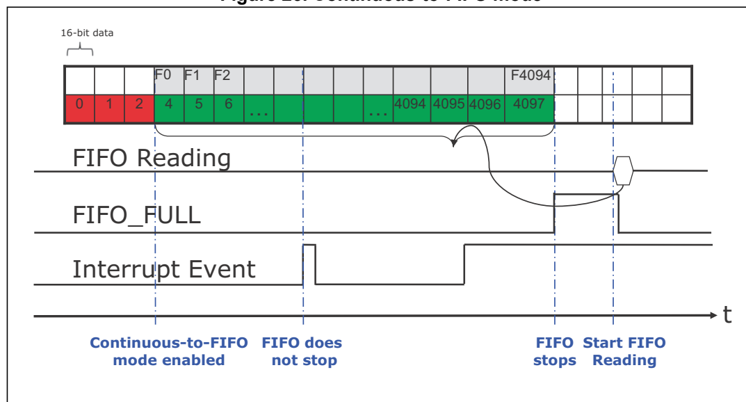
Figure 26. Continuous-to-FIFO mode
