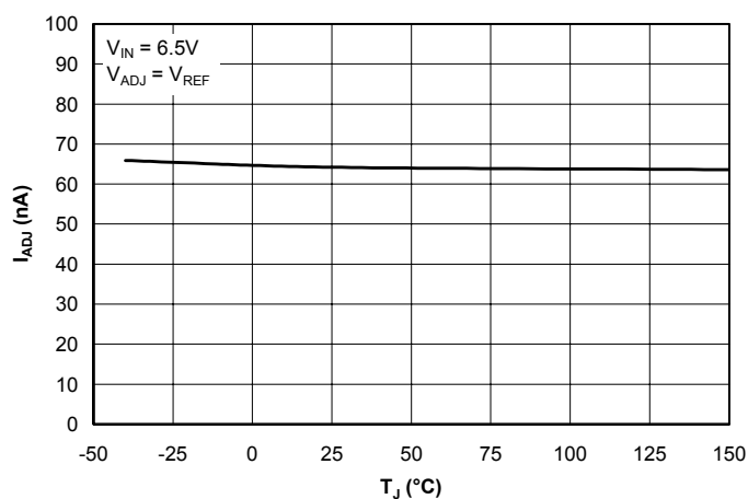
Adjust Pin Current vs. Junction Temperature
