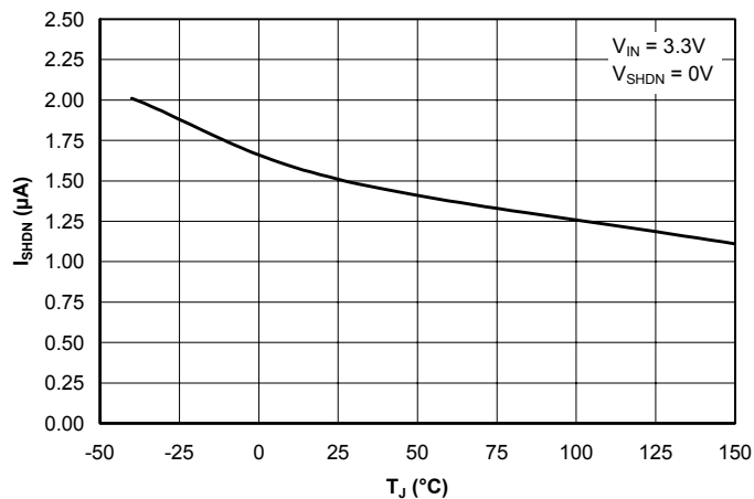
Shutdown Pin Current vs. Junction Temperature
