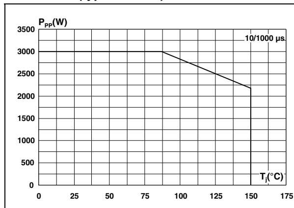
Figure 3. Peak pulse power dissipation versus initial junction temperature (typical value)
