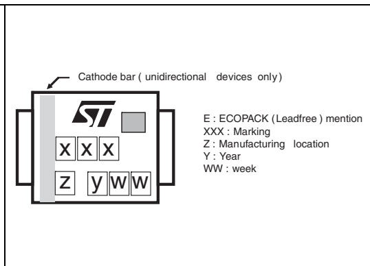
Figure 14. Marking layout (1)
