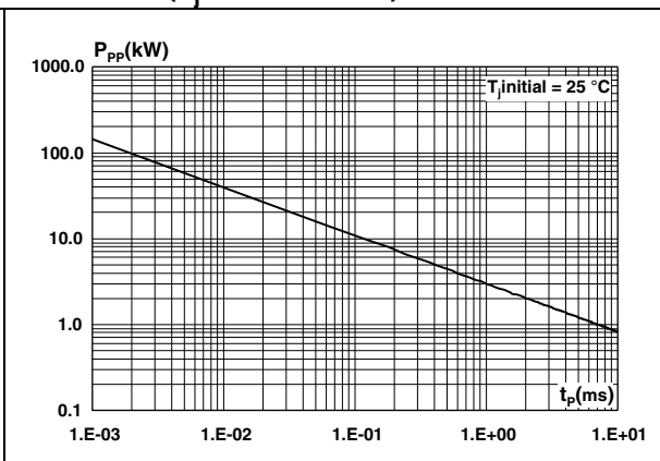
Figure 4. Peak pulse power versus exponential pulse duration ( T_{J\text{ initial}} = 25^\circ\text{C} )
