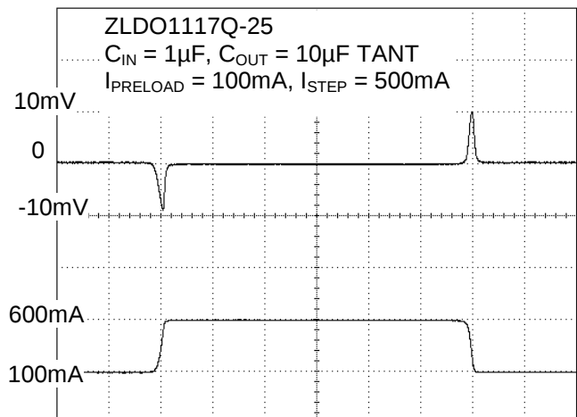
Transient Load Regulation with 10 \mu F Tantalum Capacitor
