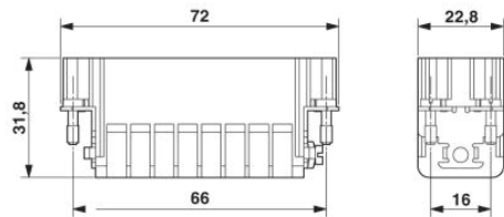
Male insert
