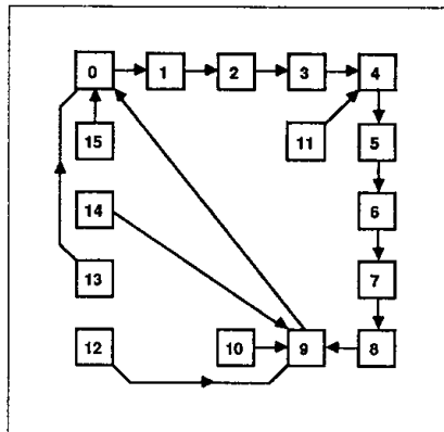
STATE DIAGRAM
