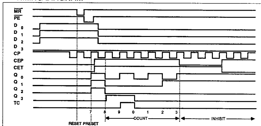
TIMING DIAGRAM
