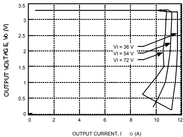
Figure 5. Typical JW050F Output Characteristics at Room Temperature
