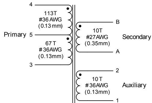
Figure 8. Flyback Transformer Schematic
