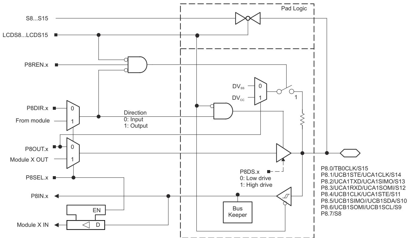
图 9-22. Port P8 (P8.0 to P8.7) Diagram
