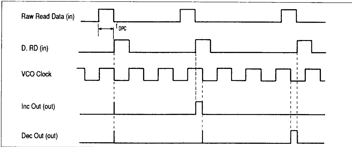
Figure 8 Phase Comparison
