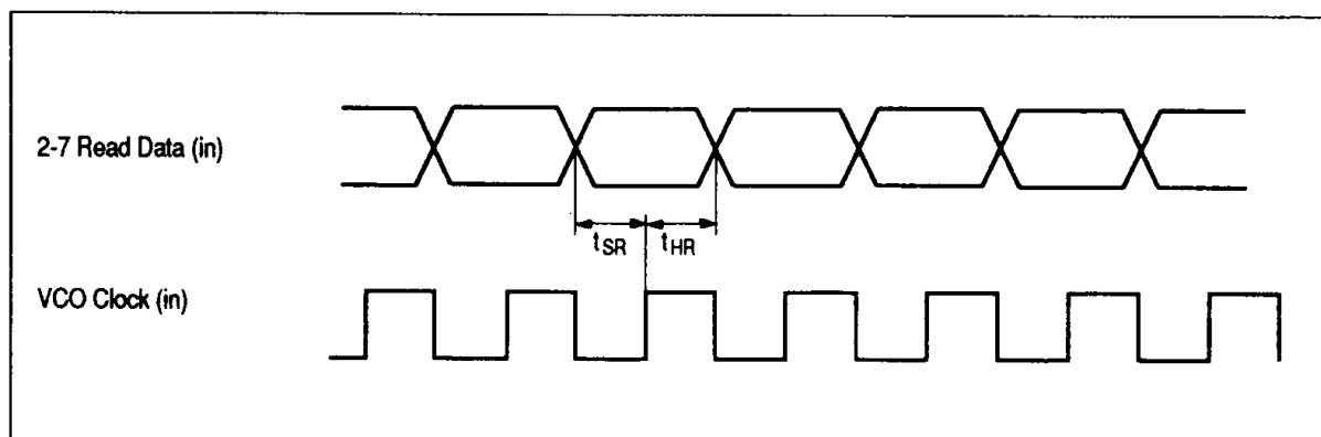
Figure 3 2-7 Read Data
