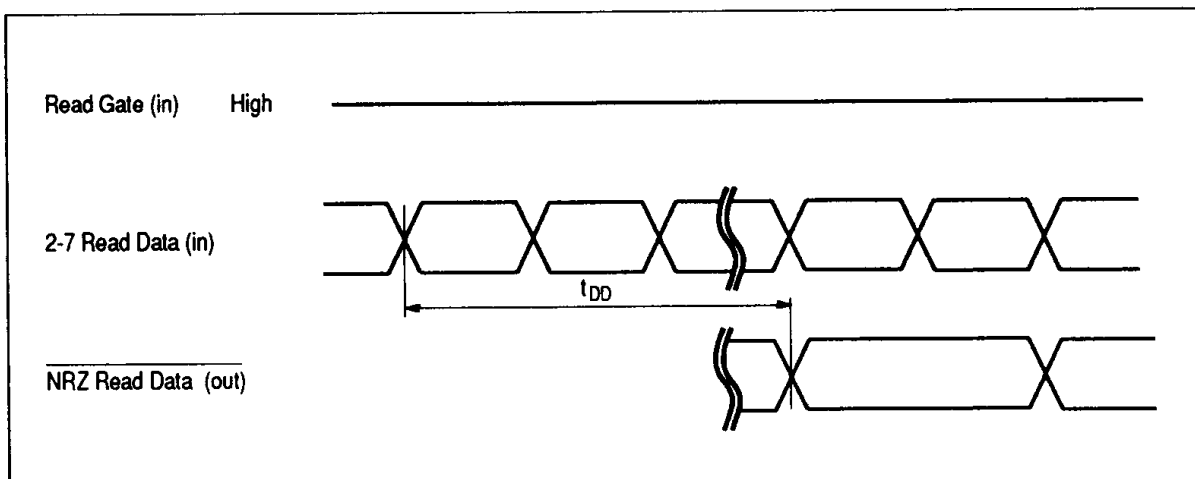
Figure 5 Decode
