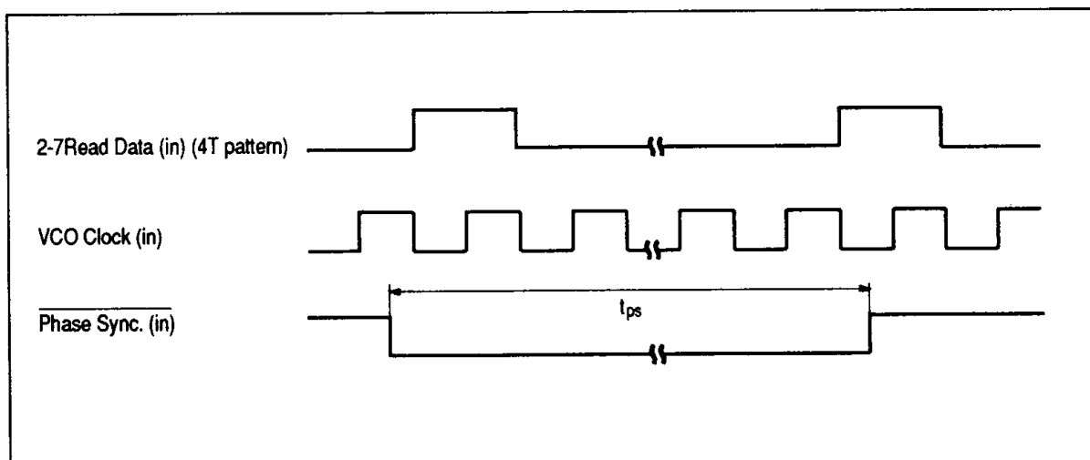
Figure 6 Phase Synchronization
