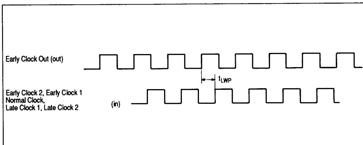
Figure 7 Write Precompensation
