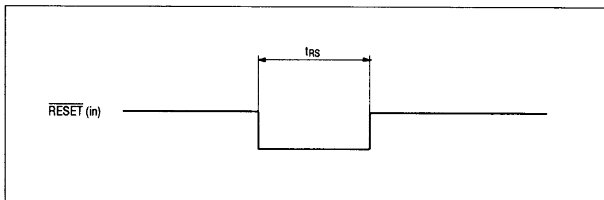
Figure 2 Reset Input
