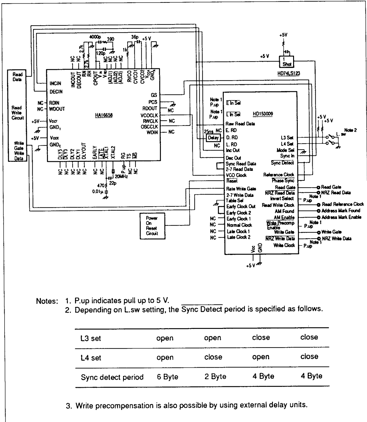
Figure 18 Circuit Example
