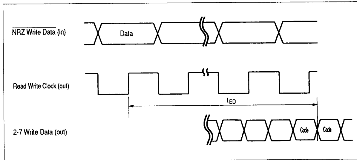
Figure 12 Encode
