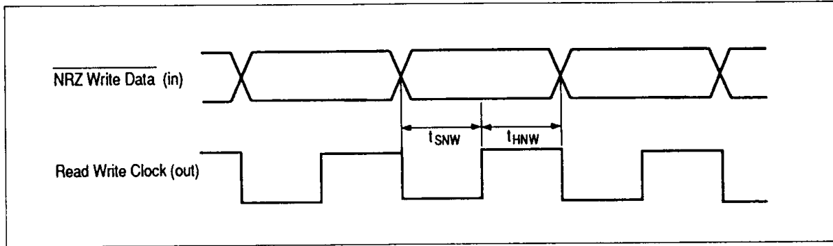
Figure 11 NRZ Write Data Input
