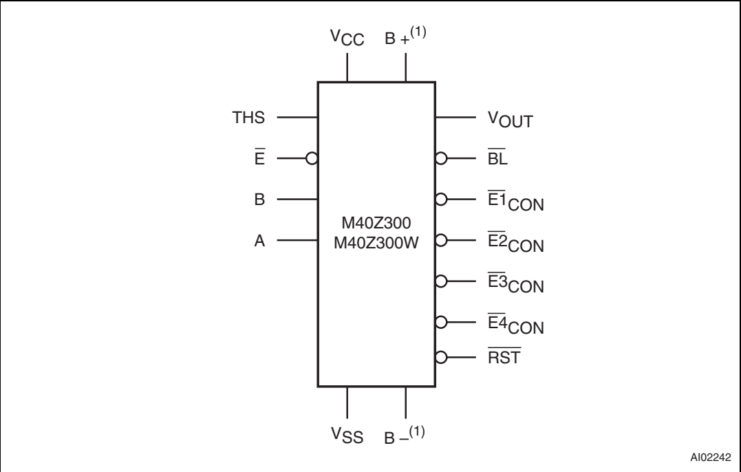
Figure 1. Logic diagram
