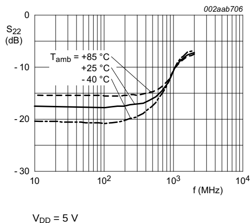
Fig 14. OFF-channel match versus frequency and temperature
