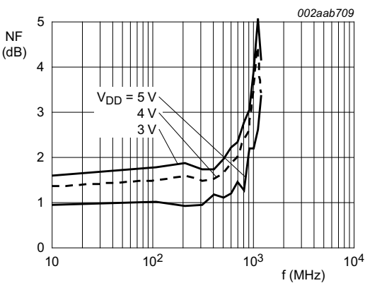
Fig 17. Noise Figure versus frequency and V_{DD}
