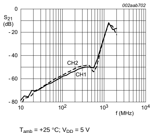
Fig 10. Isolation matching versus frequency; CH1 versus CH2
