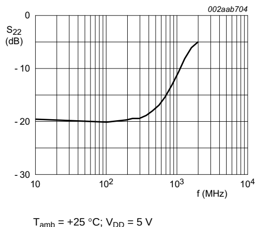
Fig 12. Output match ON-channel versus frequency
