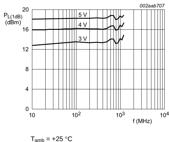
Fig 15. P_{L(1dB)} versus frequency and V_{DD}
