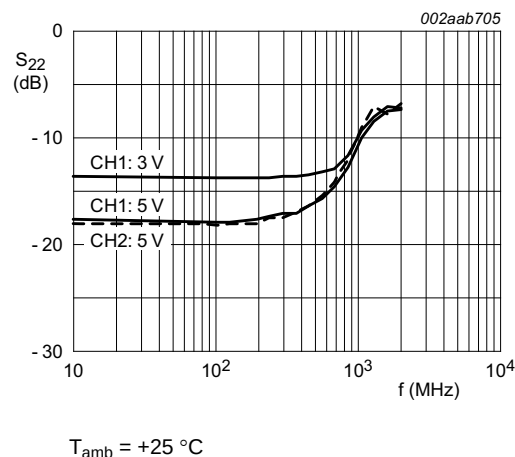
Fig 13. OFF-channel match versus frequency and V_{DD}
