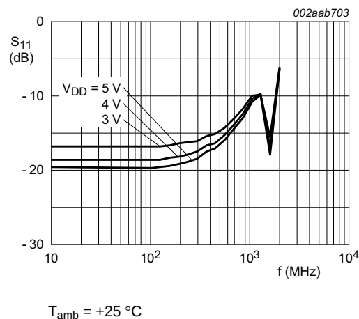
Fig 11. Input match ON-channel versus frequency and V_{DD}
