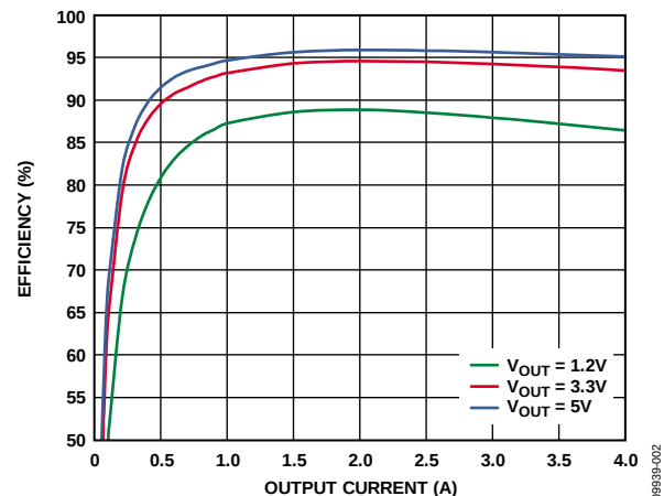
Figure 2. Efficiency vs. Output Current, V_{IN} = 12 V, f_{SW} = 250 kHz
