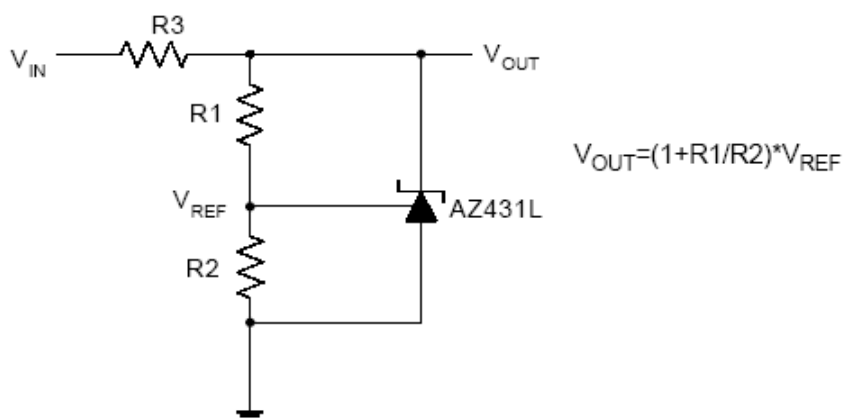
Shunt Regulator
