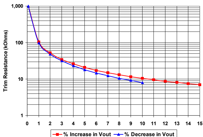
Figure C: Trim Graph for 2.5V out module
