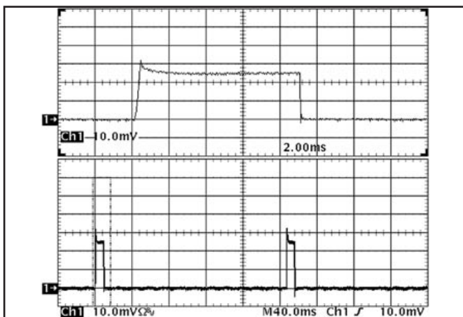
Figure 18: Load current (10A/div) as a function of time when the converter attempts to turn on into a 1 m \Omega short circuit. Top trace (2ms/div) is an expansion of the on-time portion of the bottom trace.
