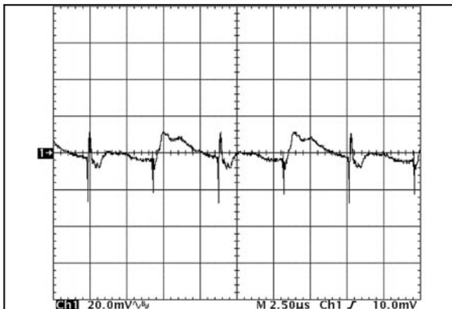
Figure 16: Output voltage ripple at nominal input voltage and rated load current (20 mV/div). Load capacitance: 1 \mu F ceramic capacitor and 15 \mu F tantalum capacitor. Bandwidth: 20 MHz. (See Figure 13)
