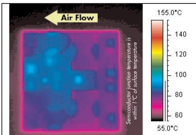
Figure 6: Thermal plot of converter at 20 amp load current with 55°C air flowing at the rate of 200 LFM. Air is flowing across the converter from output to input (nominal input voltage).
