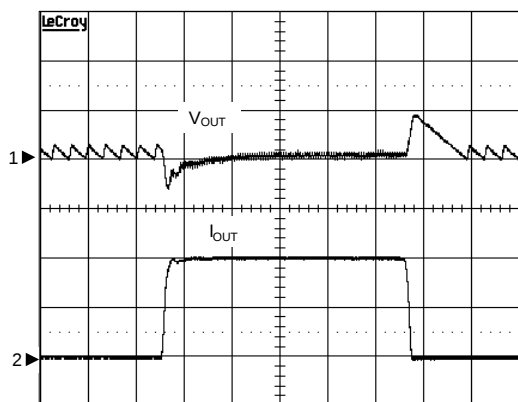
Load Transient
