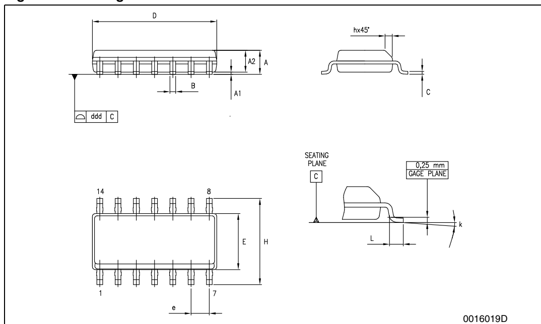
Figure 56. Package dimensions
