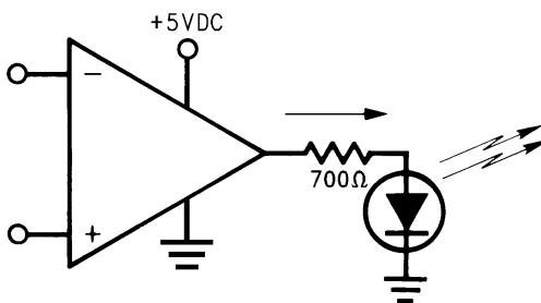
Figure 71. LED Driver
