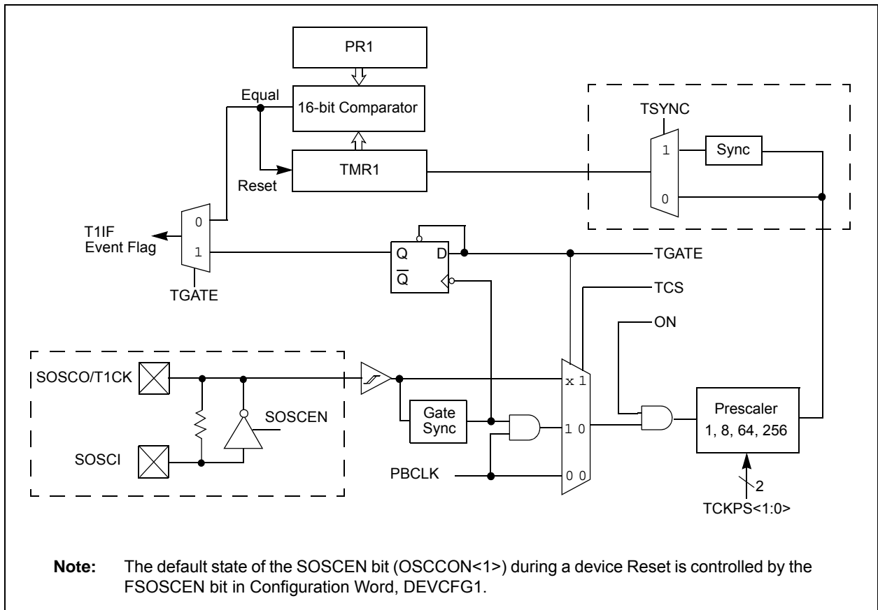
FIGURE 12-1: TIMER1 BLOCK DIAGRAM
