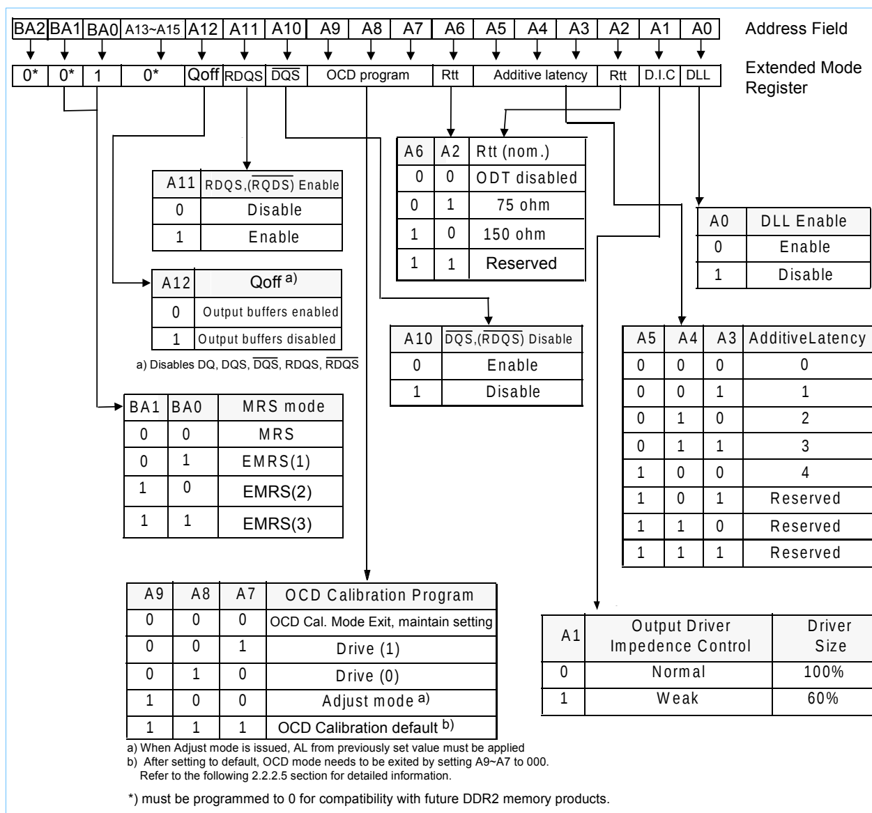
EMRS(1) Extended Mode Register Operation Table (Address Input For Mode Set)
