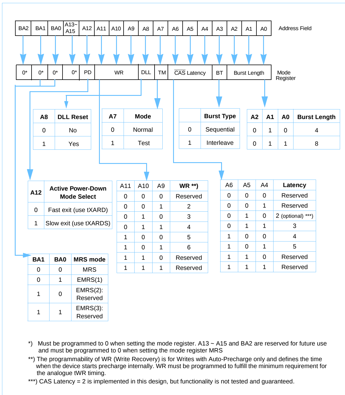
MRS Mode Register Operation Table (Address Input For Mode Set)
