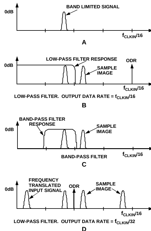
Figure 28. Band-Pass Operation
