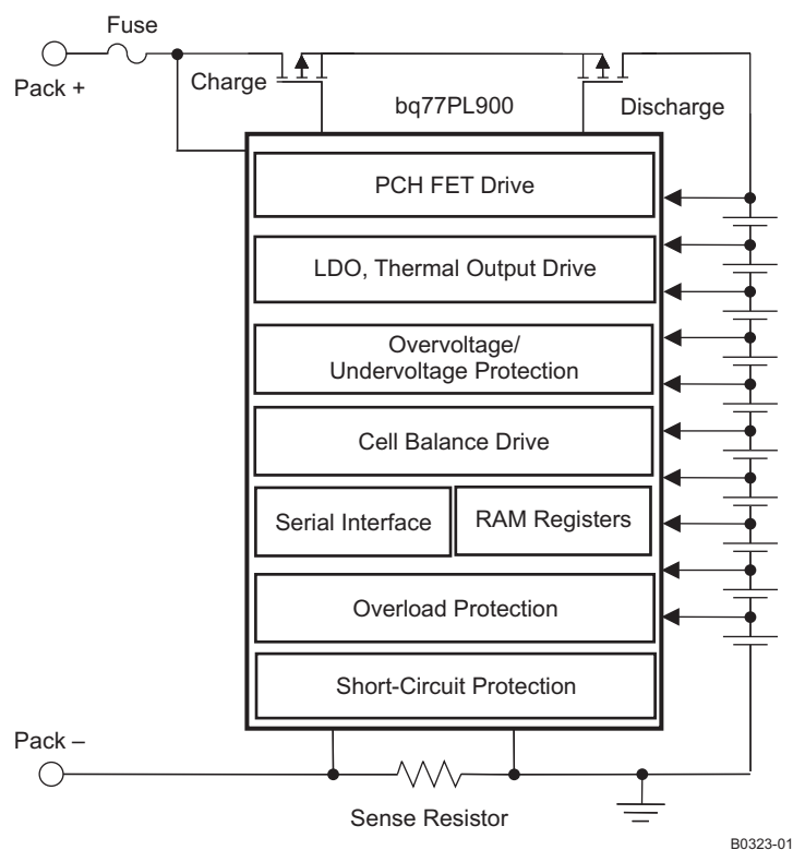
Figure 1. Stand-Alone Mode
