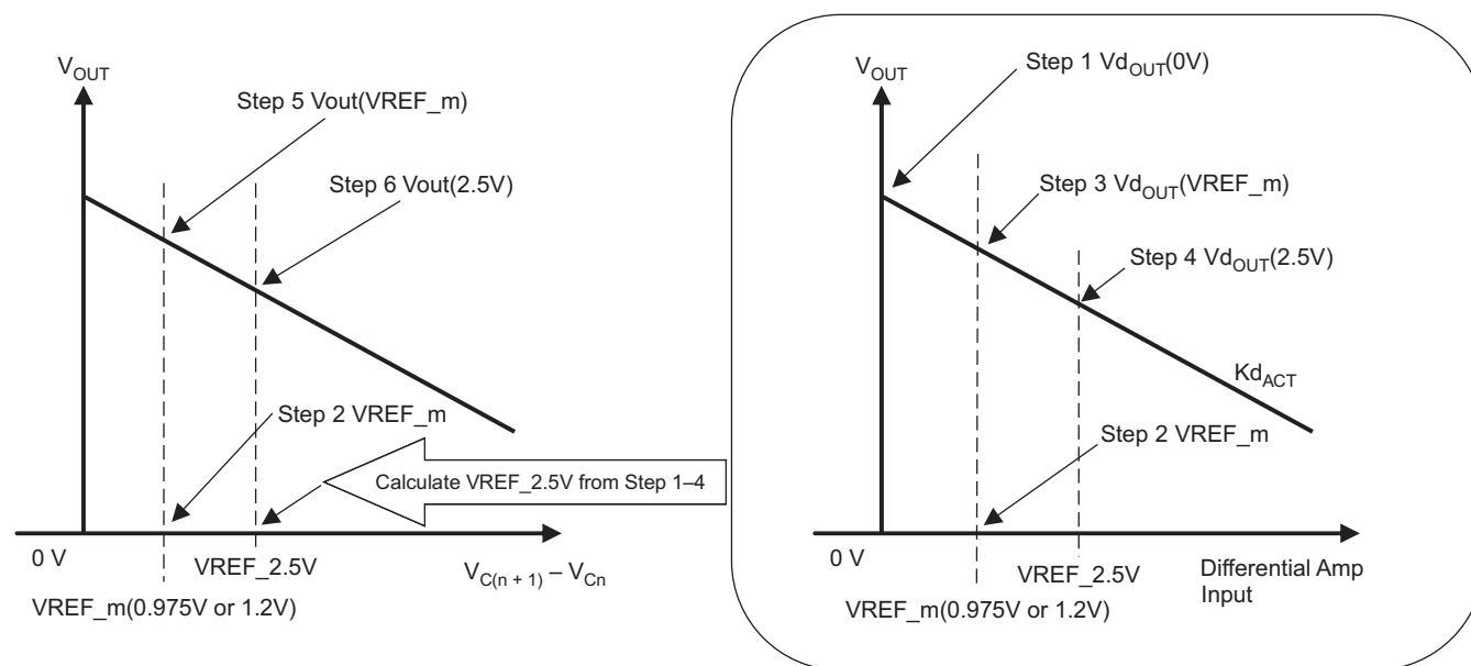
Figure 18. Calibration Method
