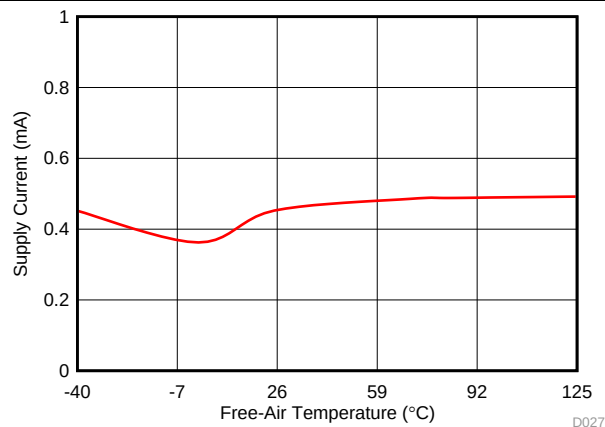
Figure 25. AVDD Current vs Temperature
