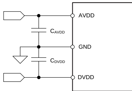
Figure 47. Power-Supply Decoupling
