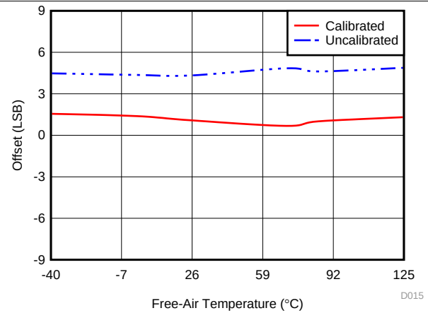
Figure 22. Offset vs Temperature
