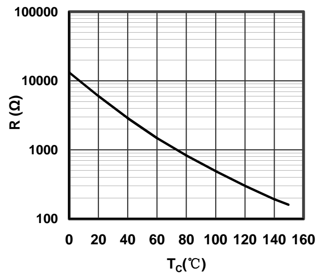
Figure 14. NTC Characteristics
