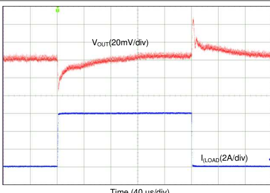
Figure 102. Transient Load Step Response, AUTO Mode (1-Phase Output)
