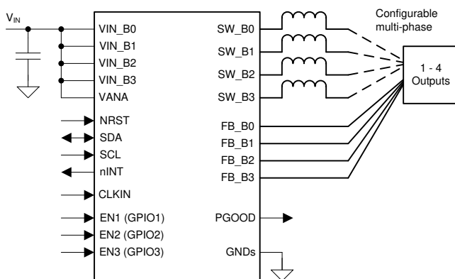
Simplified Schematic
