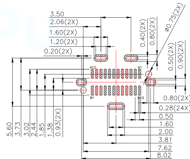
RECOMMENDED PCB LAYOUT(TOP VIEW) THICKNESS 0.8±0.10MM;DEFAULT TOLERANCE:±0.05
