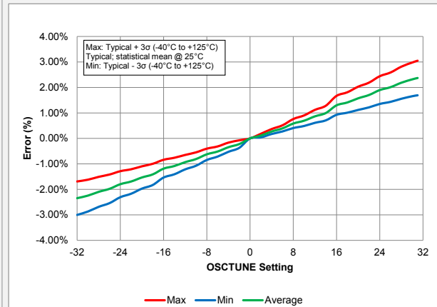
Figure 41-78. OSTUNE Center Frequency
