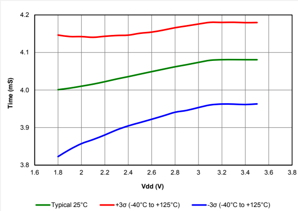
Figure 41-107. Watchdog Timer Time-out Period, PIC18LF65/66K40 only
