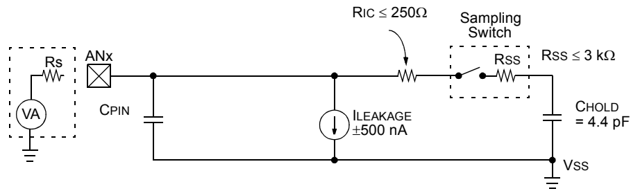
FIGURE 24-3: 10-BIT ADC MODULE ANALOG INPUT MODEL
