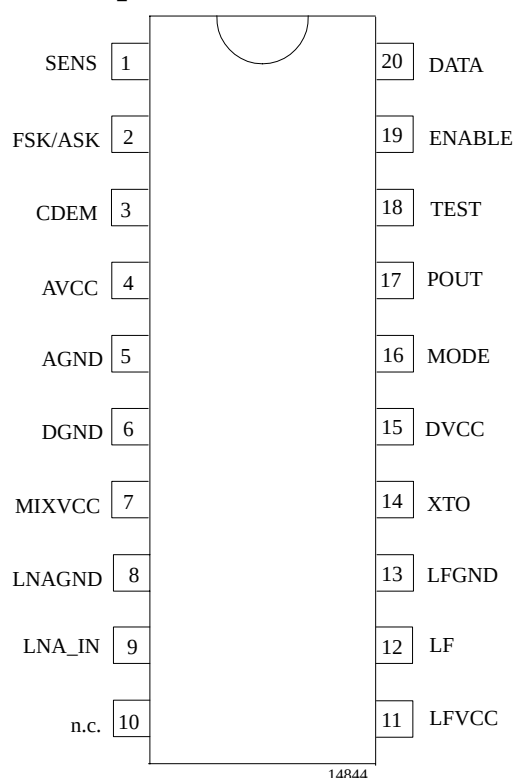
Figure 2. Pinning SO20
