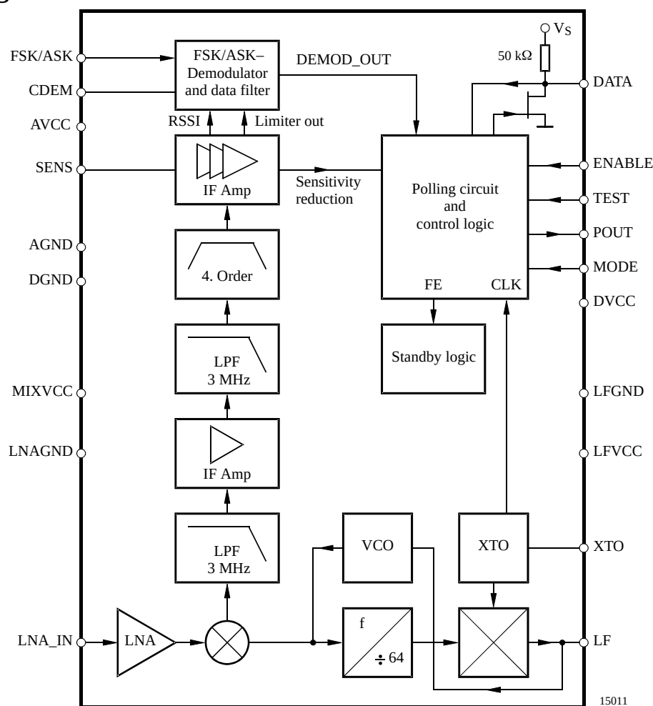
Figure 3. Block diagram
