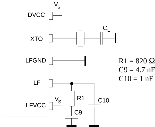
Figure 4. PLL peripherals
