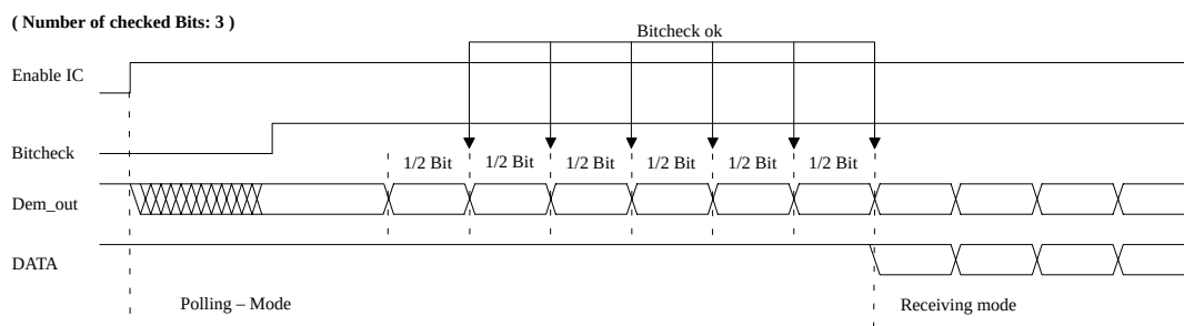
Figure 11. Timing diagram for complete sucessful bitcheck
