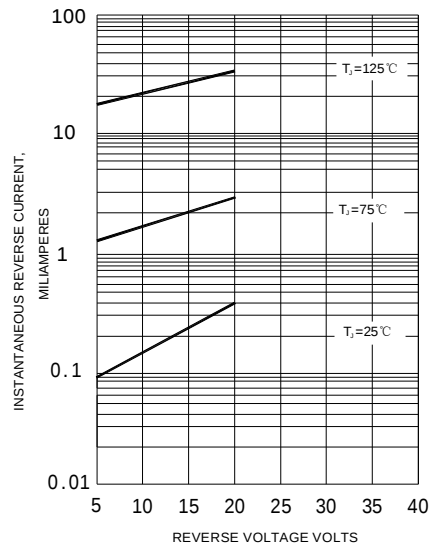
FIG.2-TYPICAL REVERSE CHARACTERISTICS
