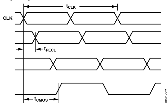
Figure 2. CLK/ \overline{\text{CLK}} to Clock Output Timing, M Divider = 1
