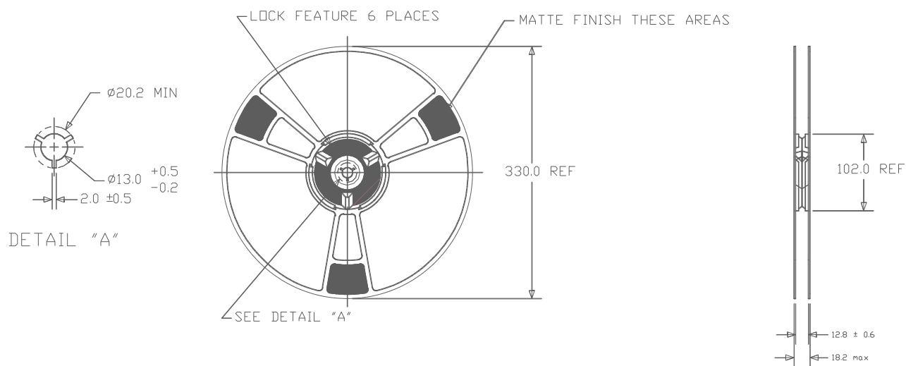
Fig.10: Outline of reel for MS5561C
