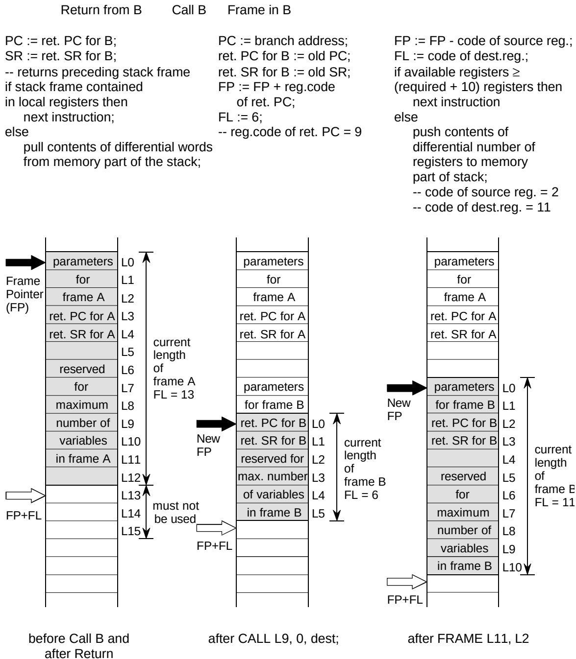
Figure 1.13: Stack frame handling (register part)
