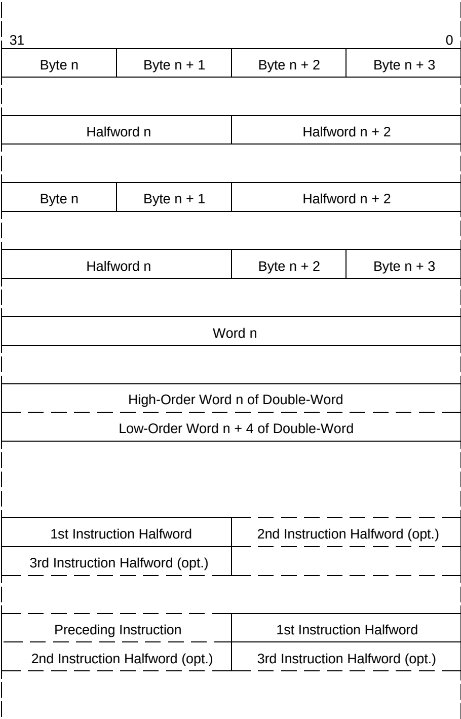
Figure 1.12: Memory Organization
