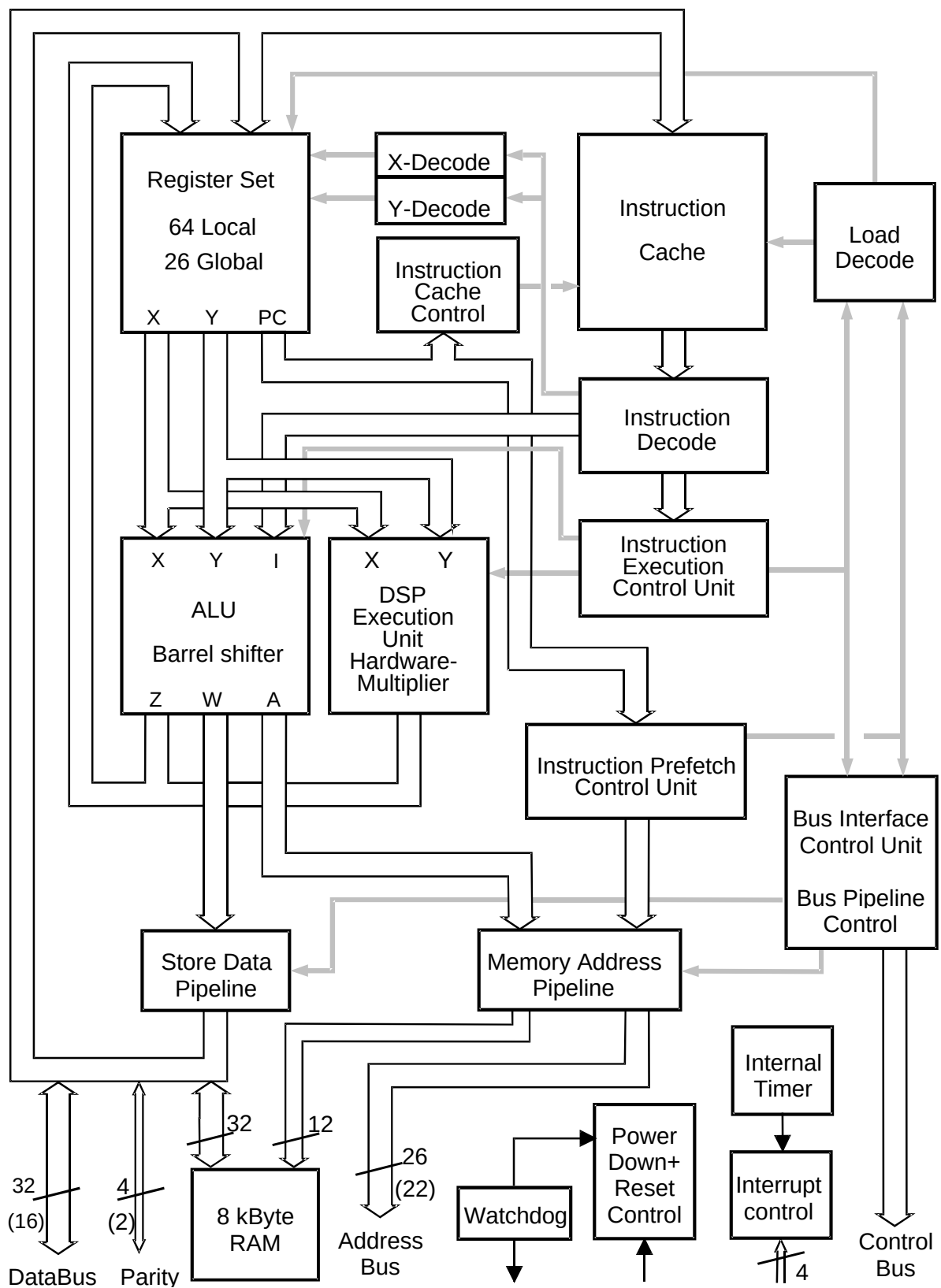
Figure 0.1: Block Diagram
