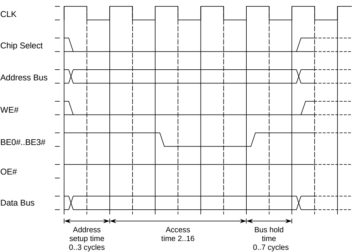
Figure 6.9: SRAM Multi-Cycle Write Access, MEMx Byte Mode = 0
