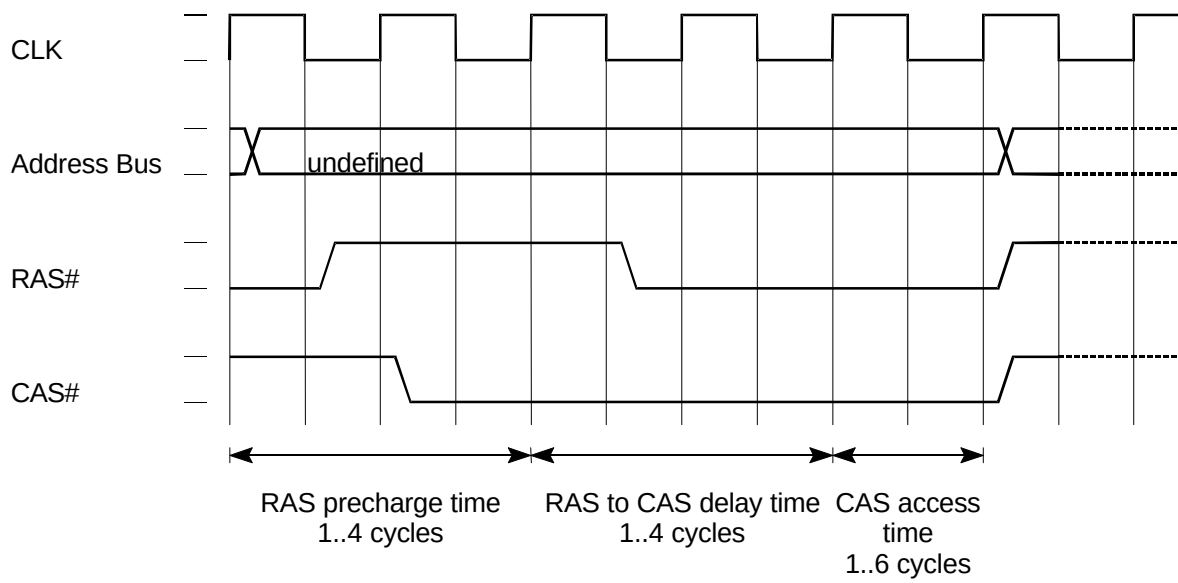
Figure 6.17: DRAM Refresh
