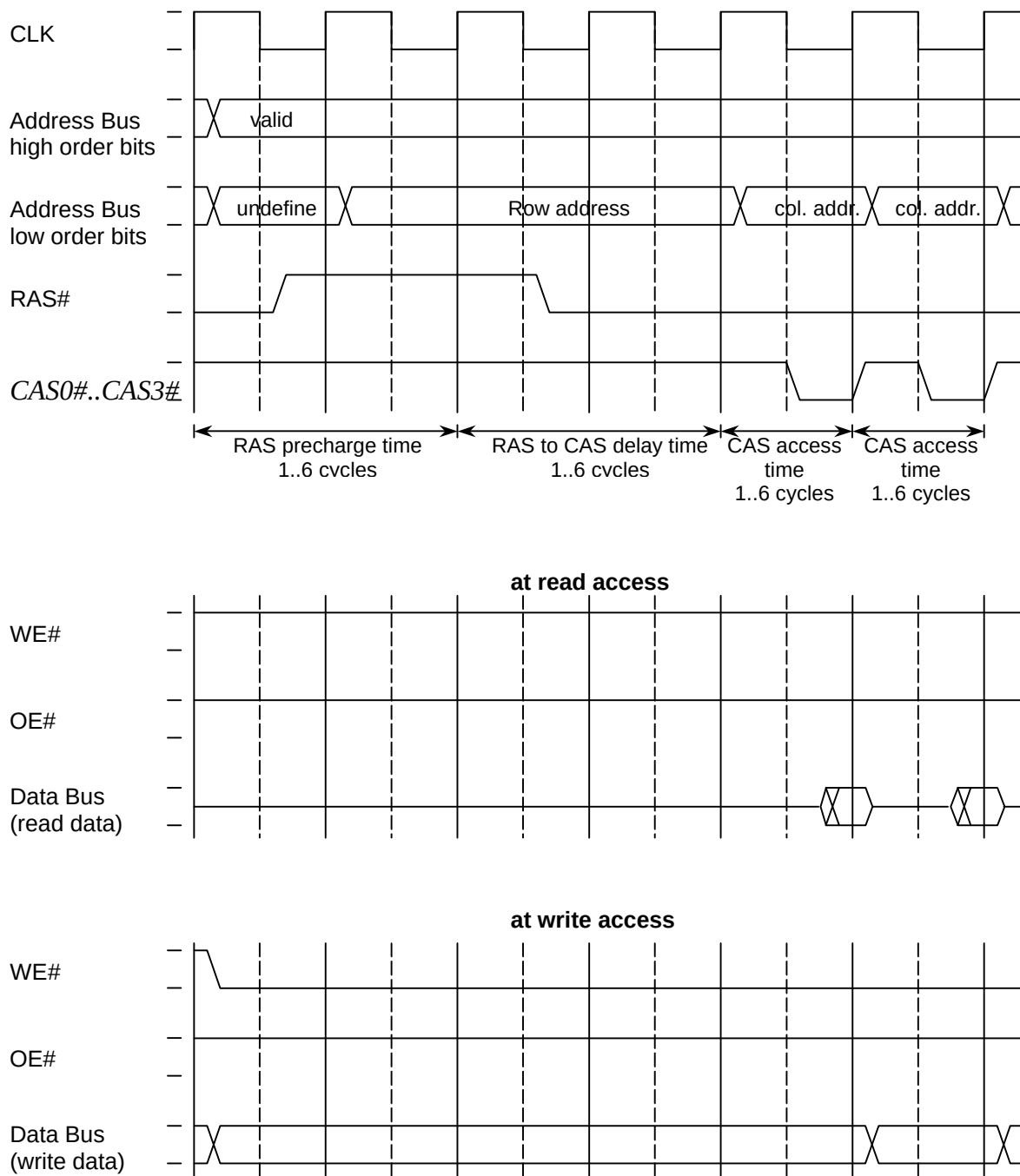
Figure 6.14: Fast Page Mode DRAM Access
