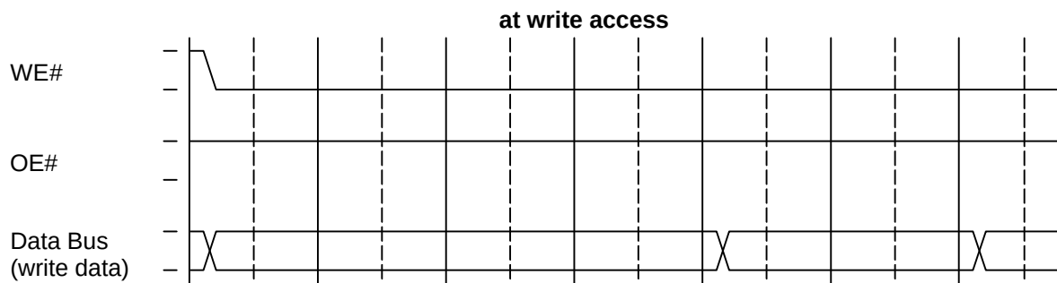
Figure 6.16: EDO DRAM Multi-Cycle Access
