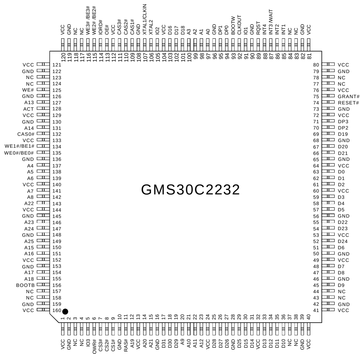
Figure 0.2: GMS30C2232, 160-Pin MQFP-Package
