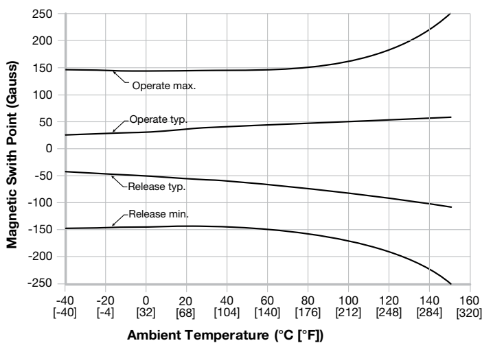
Figure 1. Magnetic Performance vs Temperature ( V_{\text{supply}} = 12 \text{ Vdc} )
