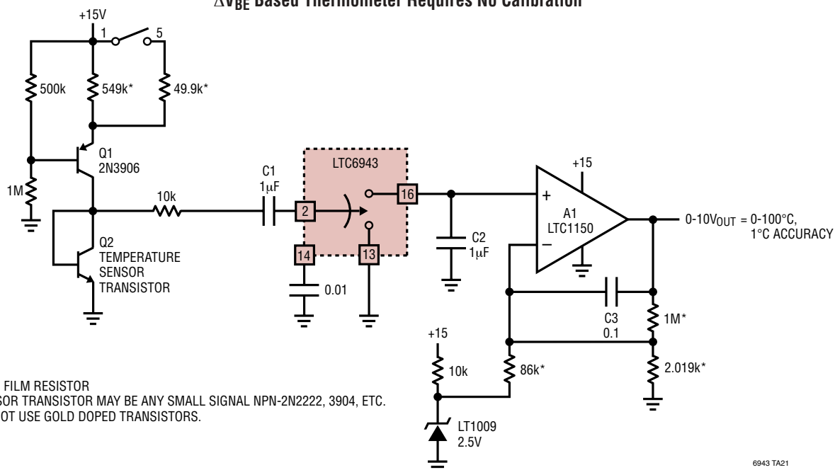
\Delta V_{BE} Based Thermometer Requires No Calibration
