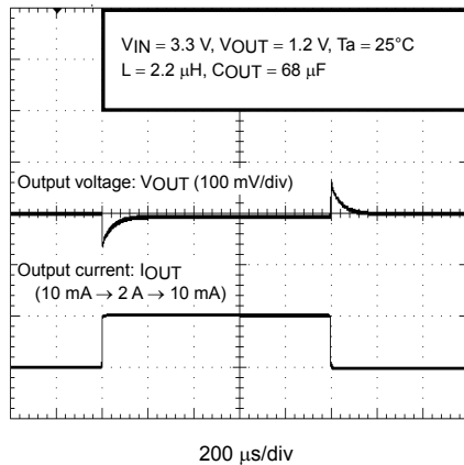
Load Response Characteristics
