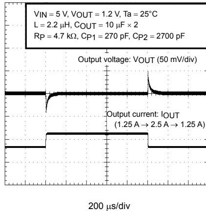
Load Response Characteristics (with an External Phase Compensation Circuit)
