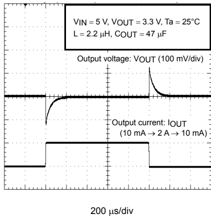
Load Response Characteristics
