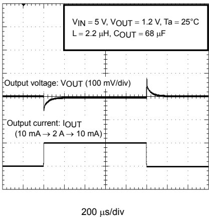
Load Response Characteristics
