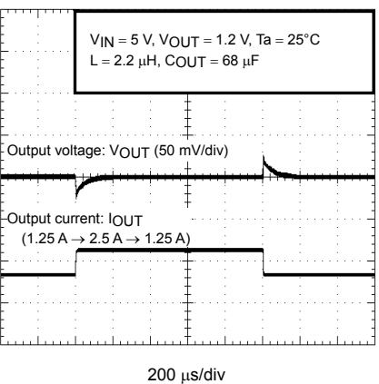
Load Response Characteristics
