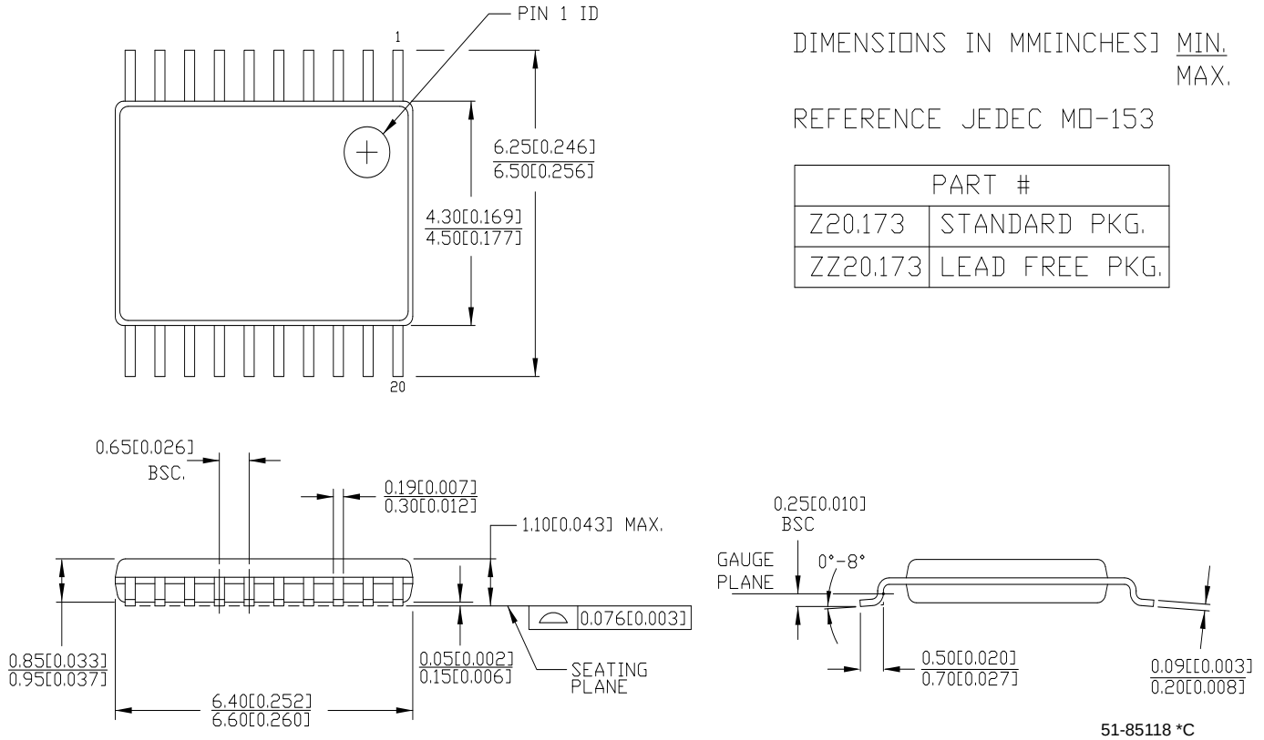
Figure 11. 20-Pin Thin Shrunk Small Outline Package (4.40 mm Body) ZZ20
