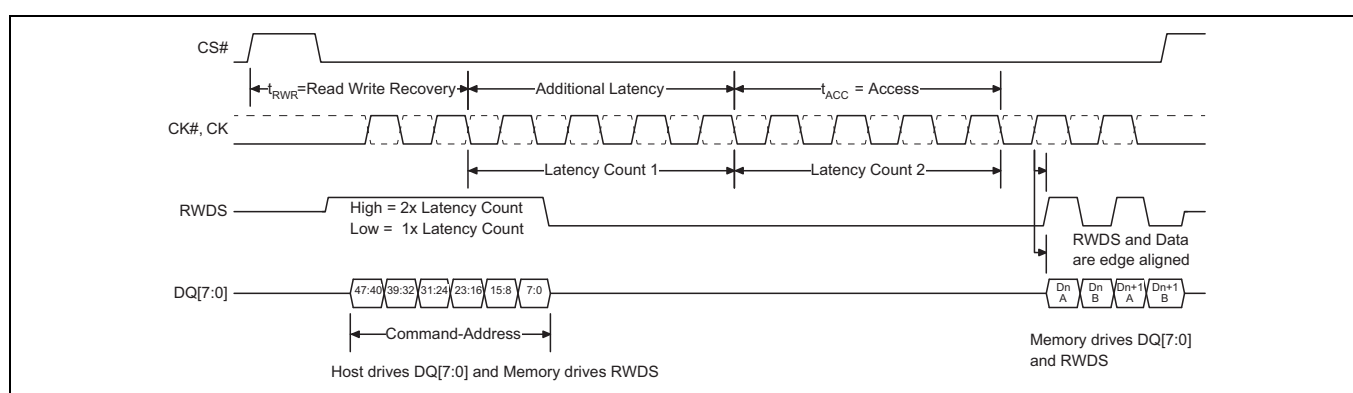
Figure 2 Read transaction
