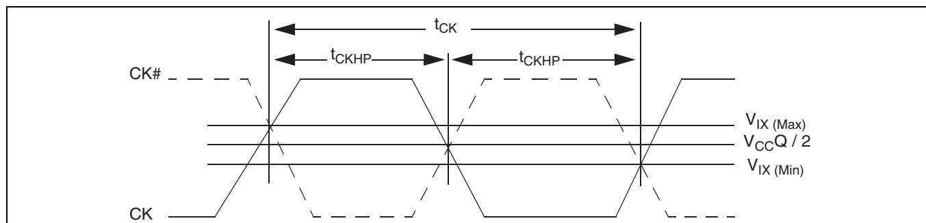
Figure 28 Clock characteristics
