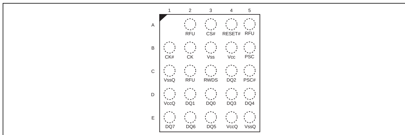
Figure 37 24-ball FBGA, 5 × 5 ball footprint, top view
