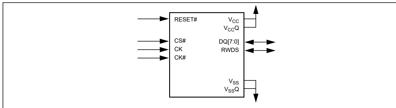
Figure 5 HYPERRAM™ interface [4]
