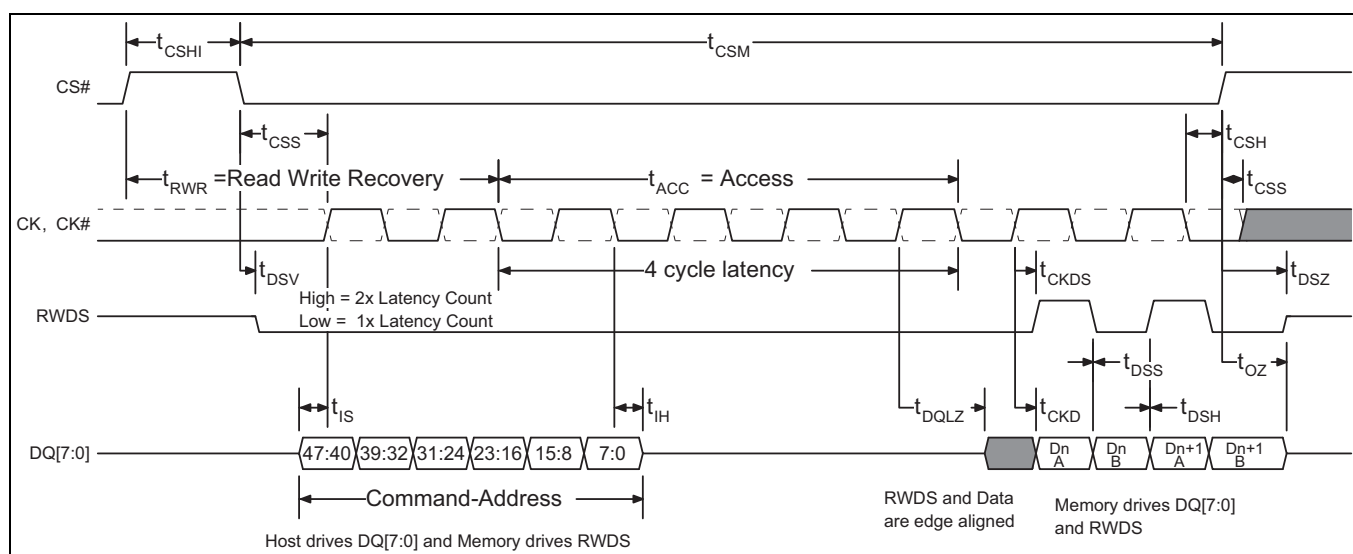
Figure 30 Read timing diagram
