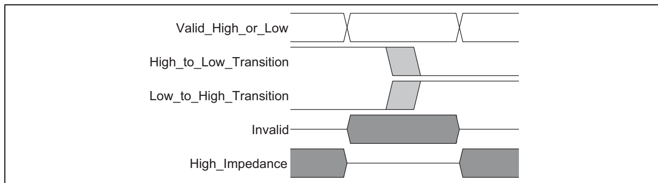
Figure 23 Switching waveforms
