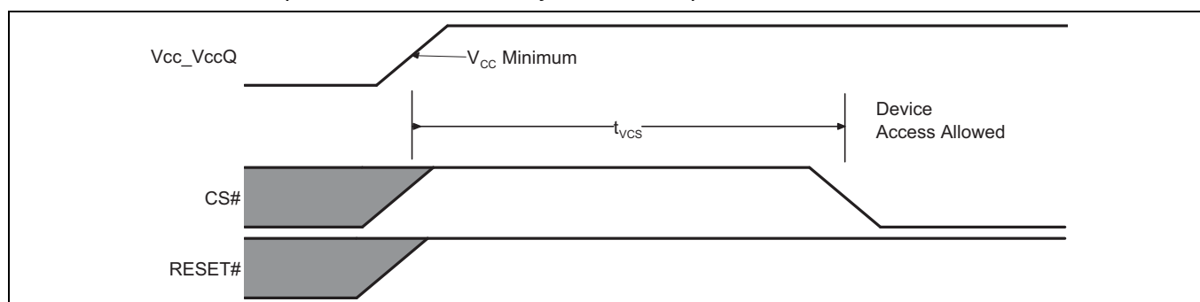
Figure 19 Power-up with RESET# HIGH
