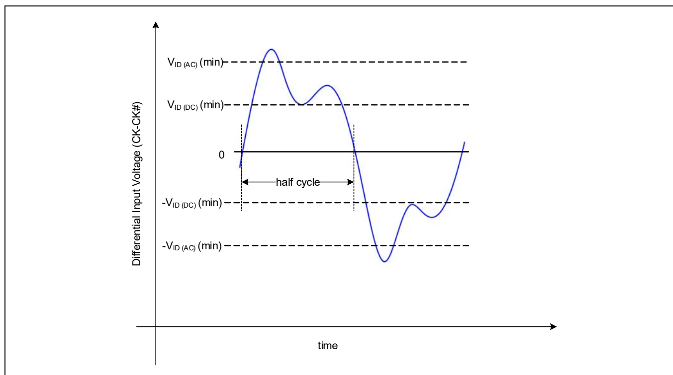
Figure 29 Differential clock (CK/CK#) input swing
