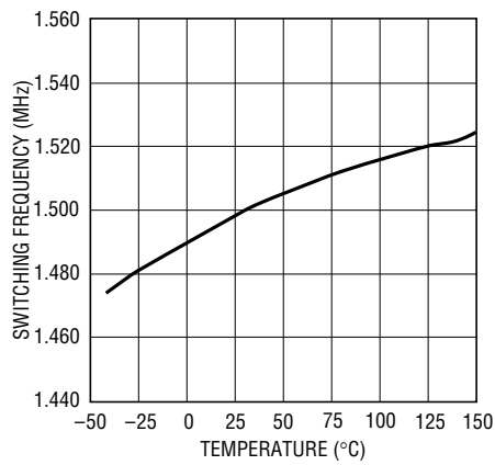
Buck Switching Frequency vs Temperature
