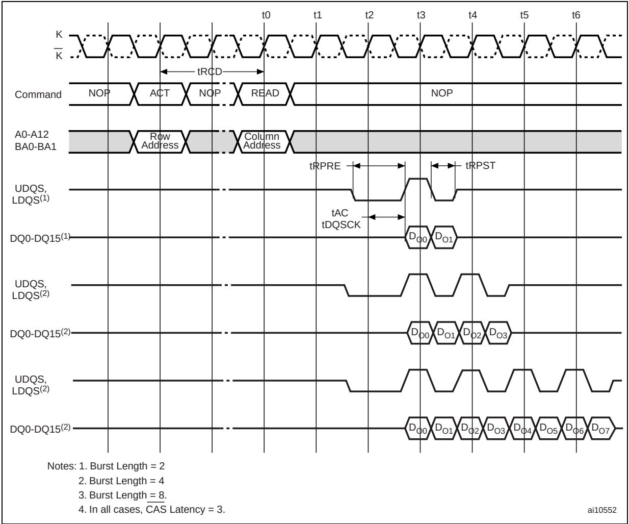
Figure 14. Read operation (Burst lengths = 2, 4 and 8, CAS latency = 3)
