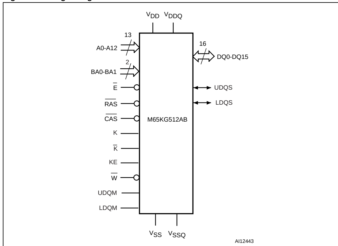
Figure 1. Logic diagram
