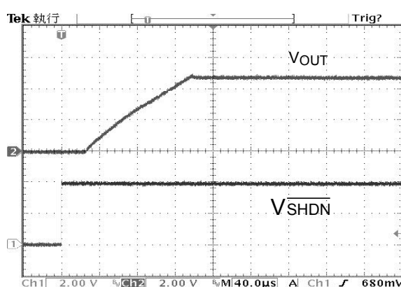
Fig. 18 Start-Up Time
