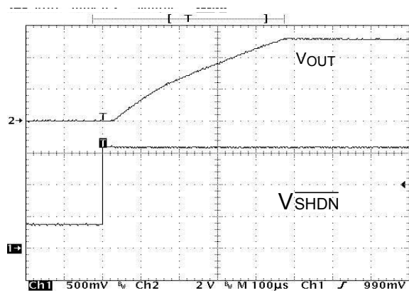
Fig. 17 Start-Up Time
