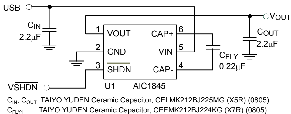
Fig. 27 Regulated 5V from USB
