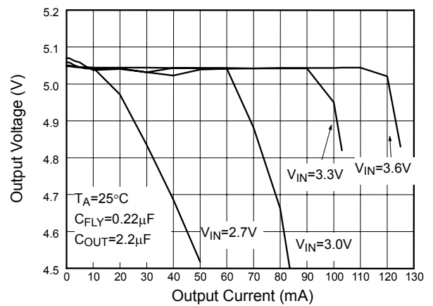
Fig. 4 Load Regulation
