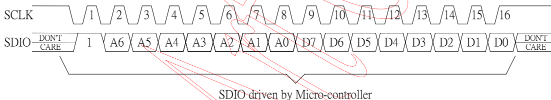
Figure 7. Write operation
