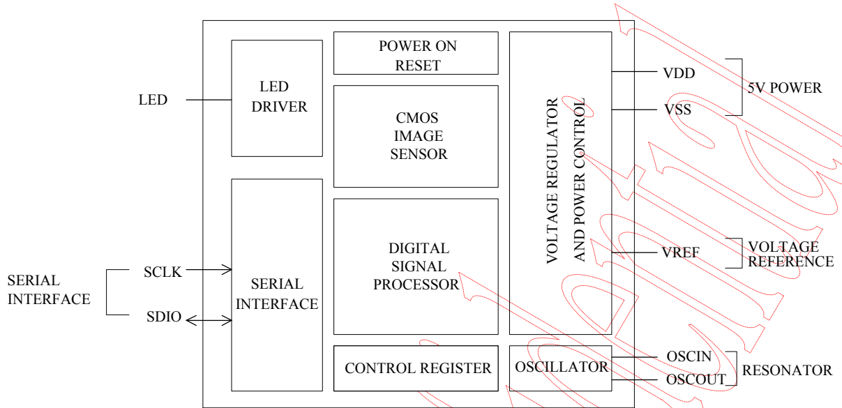
Figure 3. Block diagram
