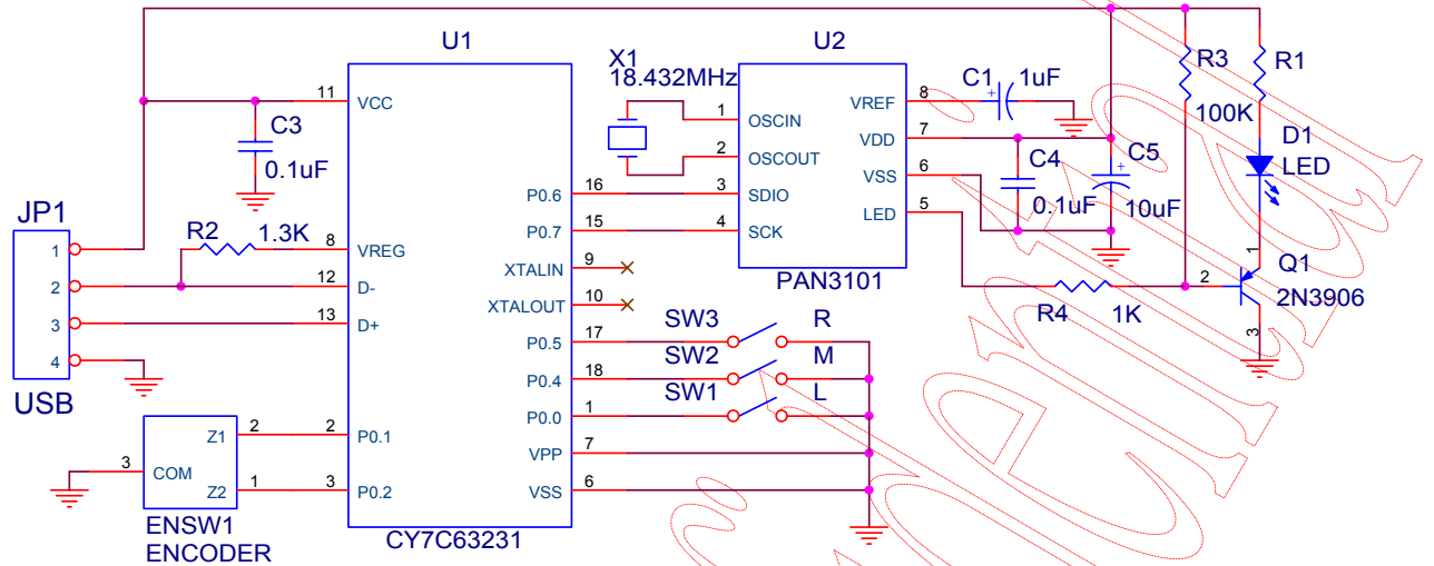
Figure 11. Application circuit using external LED
