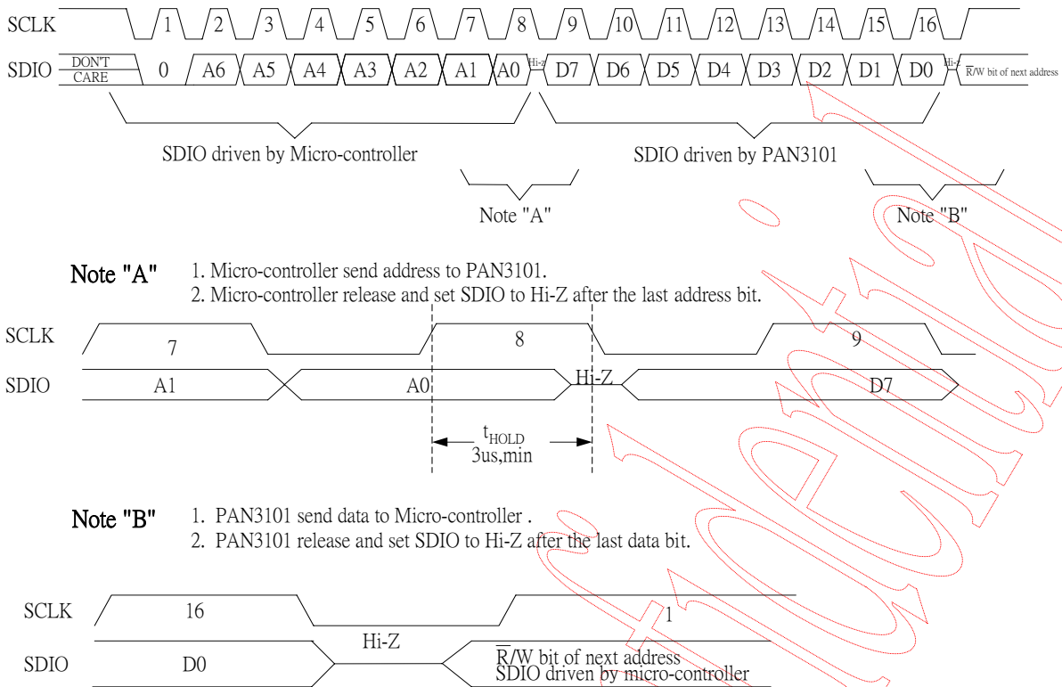
Figure 8. Read operation
