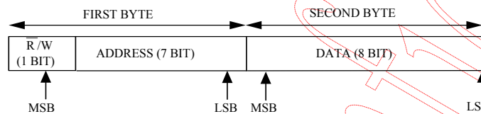
Figure 6. Transmission protocol
