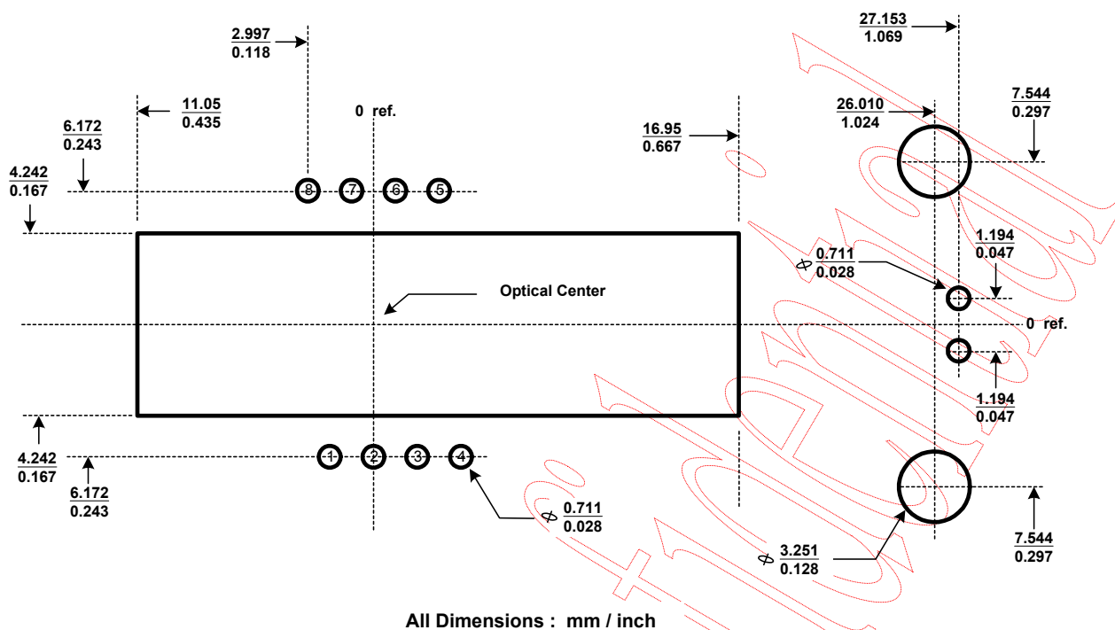
Figure 16. Recommended PCB mechanical cutouts and spacing
