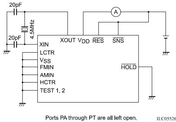
Figure 2. I_{DD3} and I_{DD4} in Backup Mode
