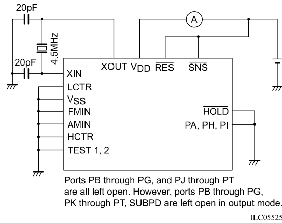
Figure 1. I_{DD2} in Halt Mode
