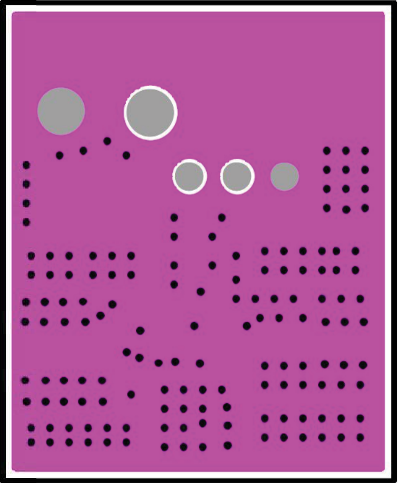
PCB Layout—Layer 3
