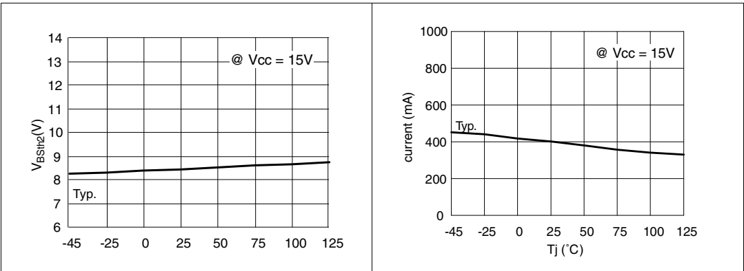
Figure 10. V_{\text{BOOT}} UV turn-off threshold vs. temperature Figure 11. Output source current vs. temperature
