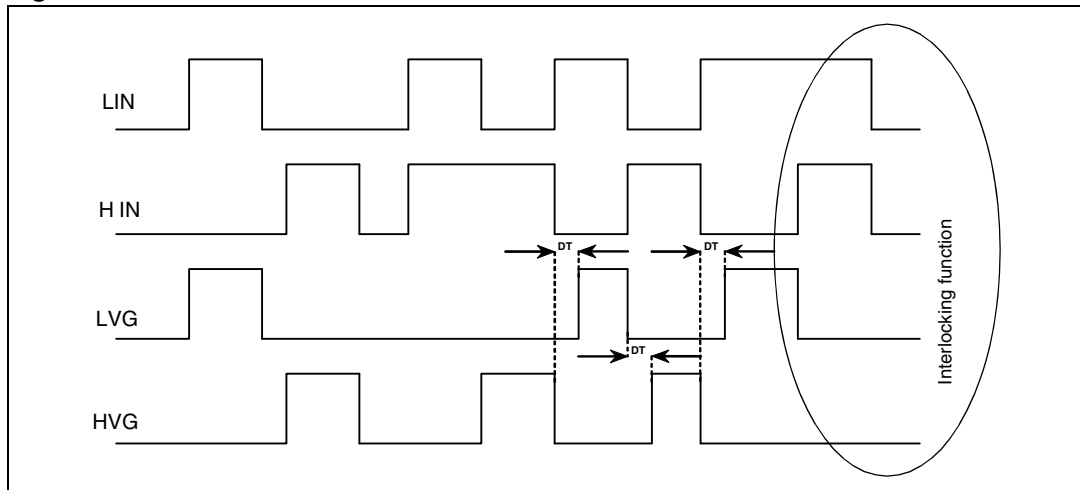
Figure 3. Dead time waveform definition
