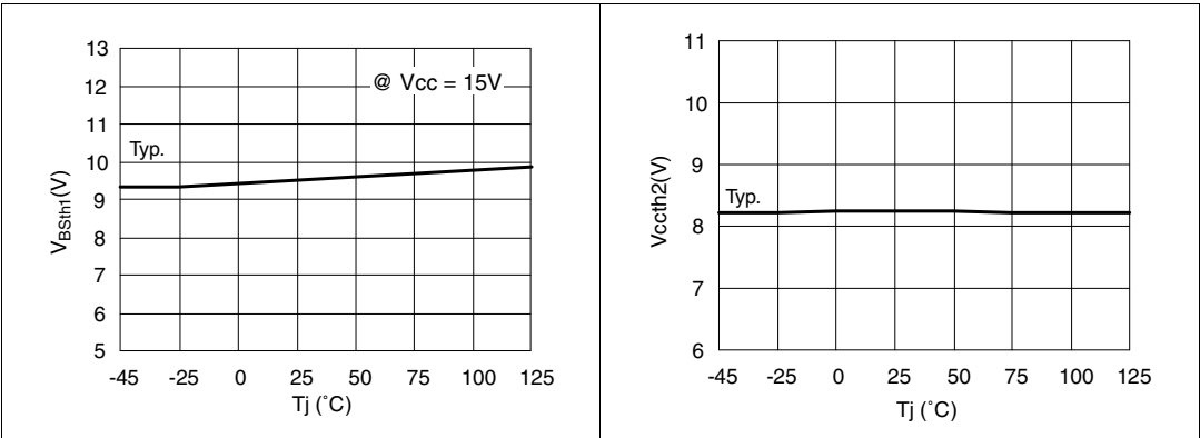
Figure 8. V_{\text{BOOT}} UV turn-on threshold vs. temperature Figure 9. V_{\text{CC}} UV turn-off threshold vs. temperature
