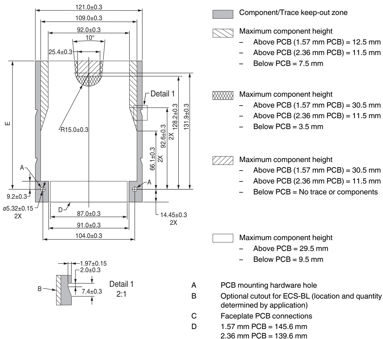
Figure 6 Circuit board design dimensions and restrictions
