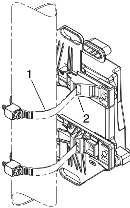
Figure 15 Hose-clamp mounting
