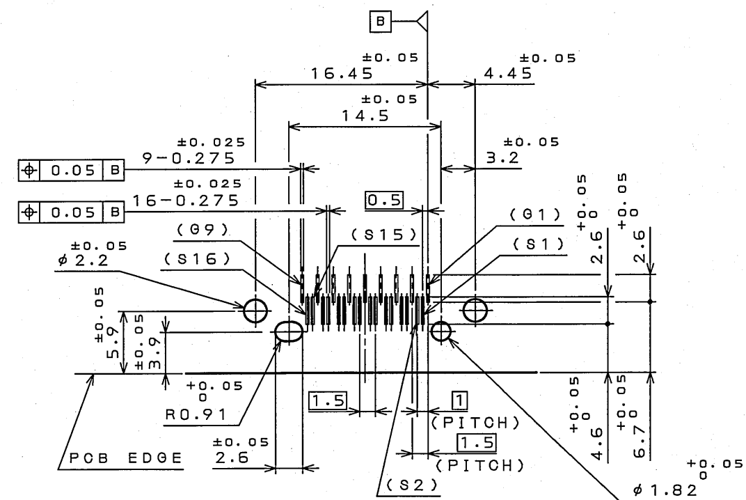
APPLICABLE P.C.B. DIMENSION(REF.)
