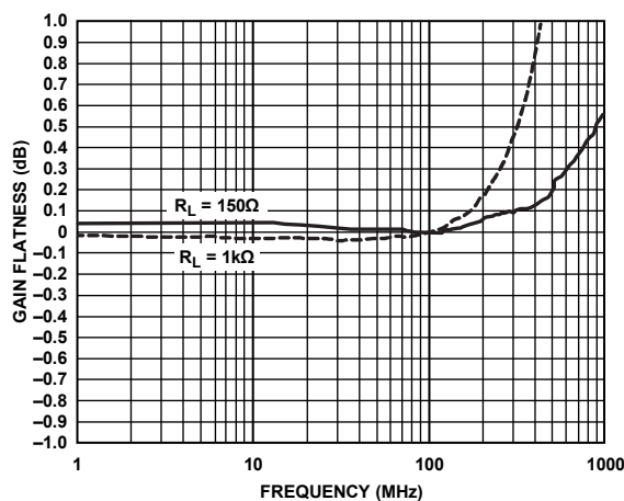
Figure 8. Gain Flatness vs. Frequency ( R_L = 150\text{ }\Omega and 1 k \Omega , A_V = 10\text{ dB} )
