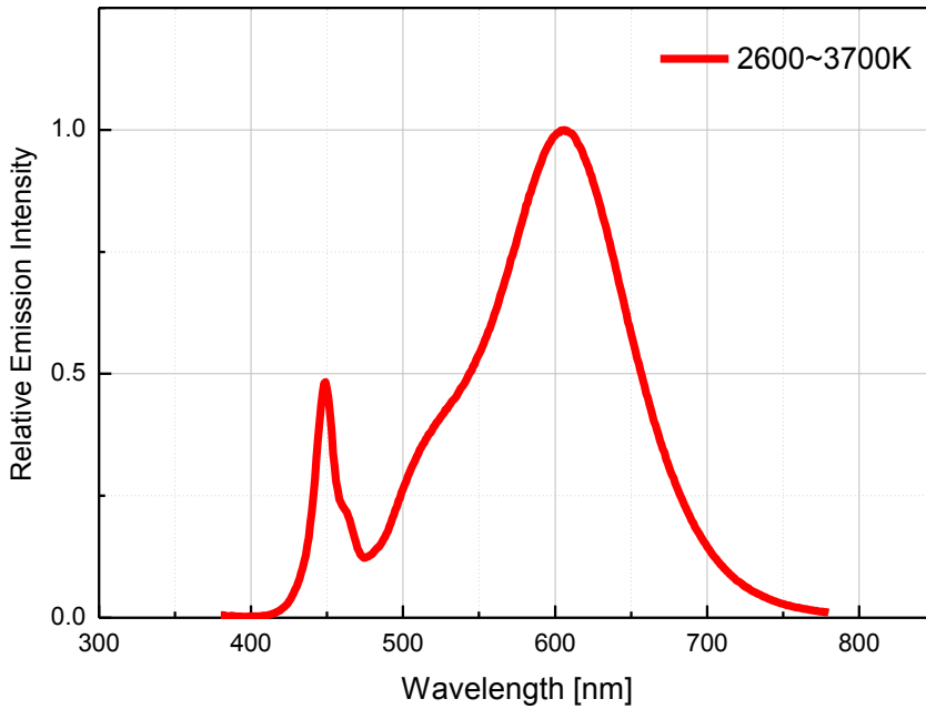
Fig 1. Color Spectrum, T_j = 25^\circ\text{C} , I_F = 100\text{mA}
